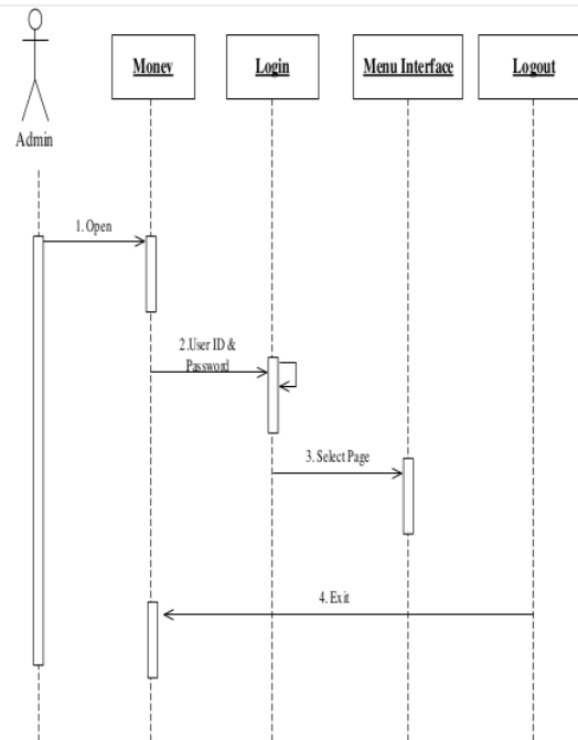
Figure 13. Sequence Diagram Money Blended Learning
