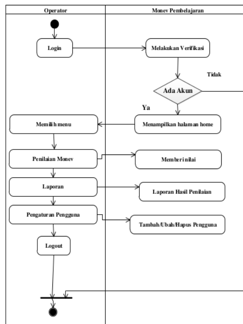
Figure 12. Activity Diagram Money Learning for Operators
