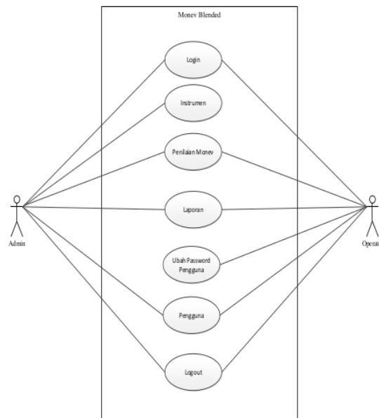
Figure 11. Usecase Diagram for Monitoring and evaluation
